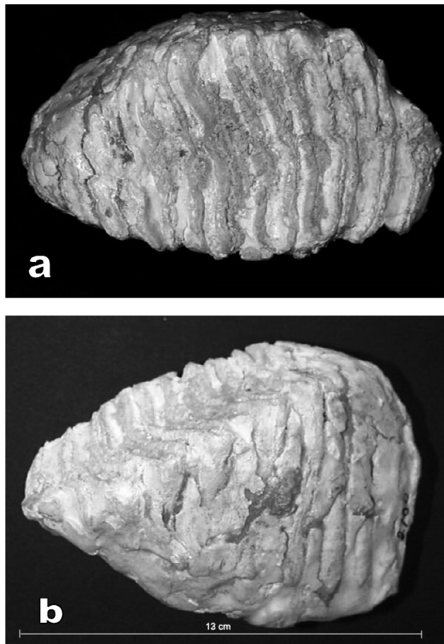
Fig.3 - Mammuthus lamarmorae (Major, 1883) from San Giovanni in Sinis: M 3 in occlusal view, approximately x0.7 of natural size.
